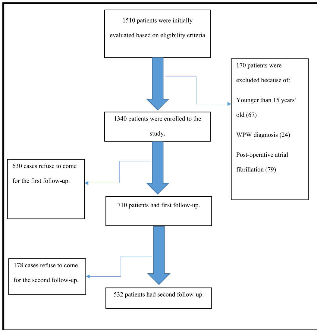
Fig. 1. Study flowchart.
